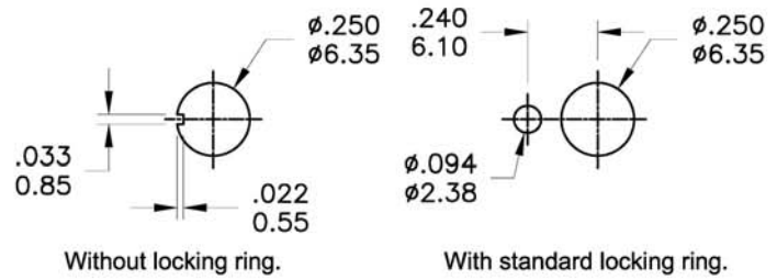
PANEL MOUNTING
