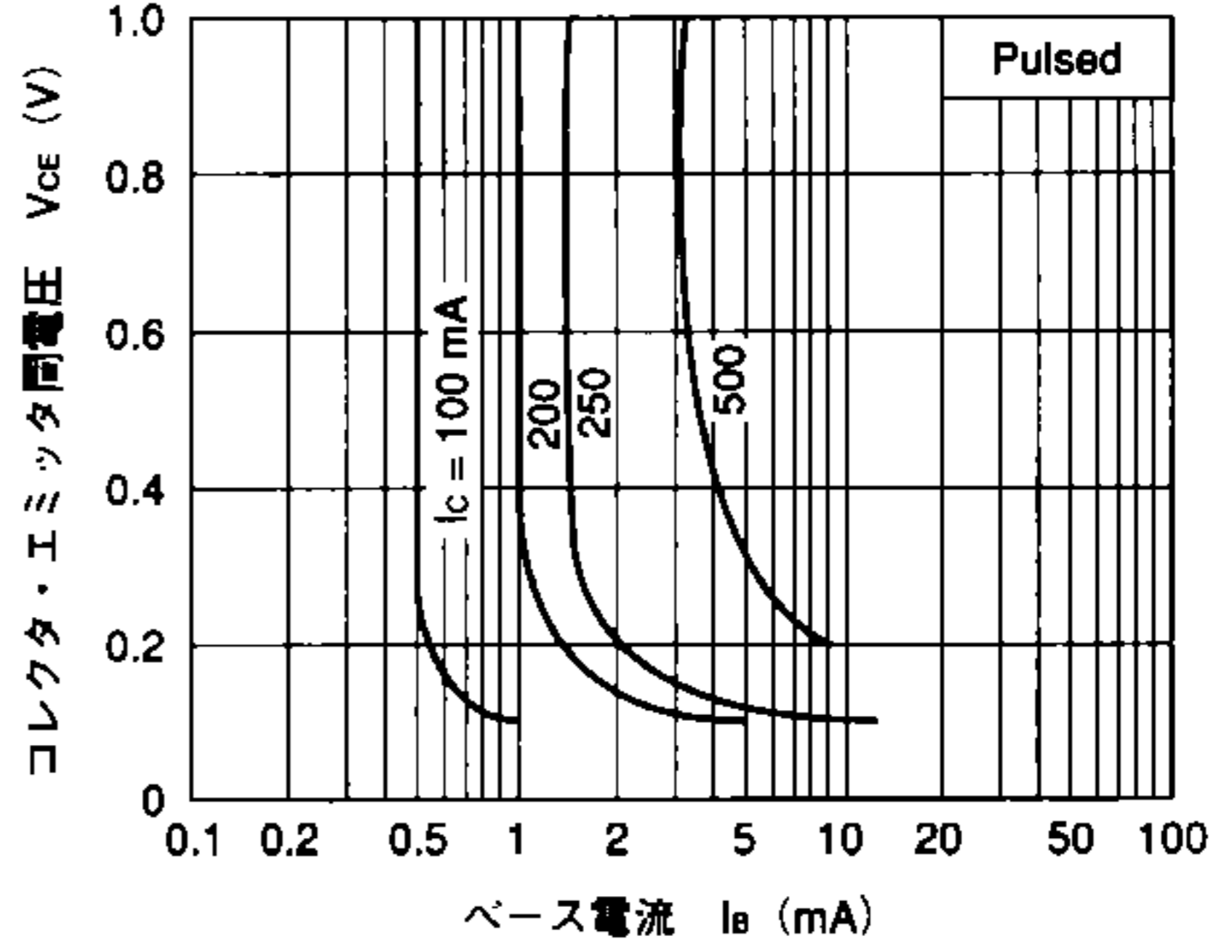
COLLECTOR TO EMITTER VOLTAGE vs. BASE CURRENT
