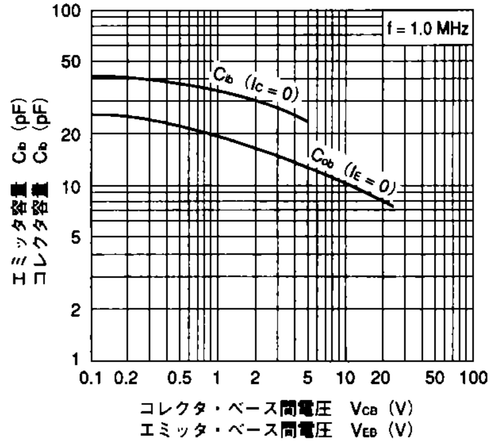
INPUT AND OUTPUT CAPACITANCE vs. REVERSE VOLTAGE
