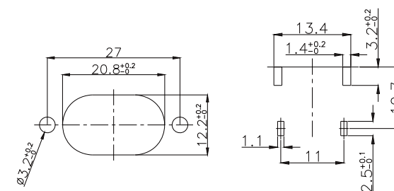
取付穴参考図 Size of mounting hole
