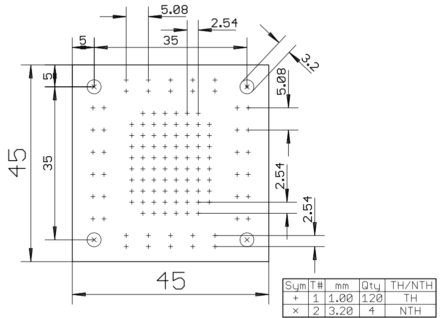
AE-DIP20-UNIV45X45
