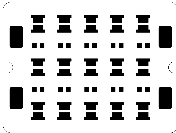
AE-LEDLAMP-SUNWHITE-5x3 L1MASK
