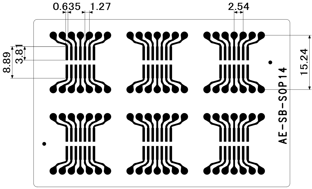
AE-SB-SOP14
