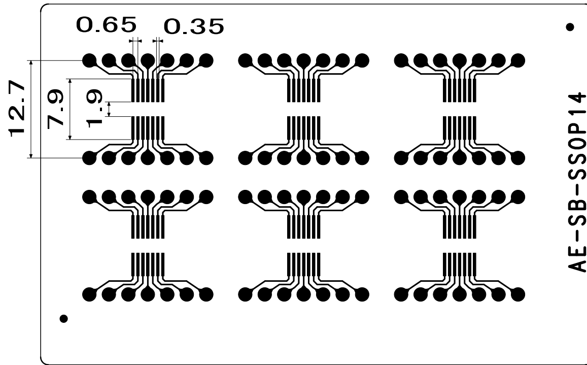
AE-SB-SSOP14
