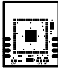
AE-ESP32-PICO-V3-ZERO TOP-SOLDERMASK
