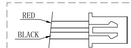
JST XHP-2P HOUSING BACK VIEW S=2
