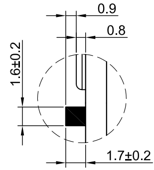
POLARITY PROTECTION DEVICE DETAIL "A" S=3
