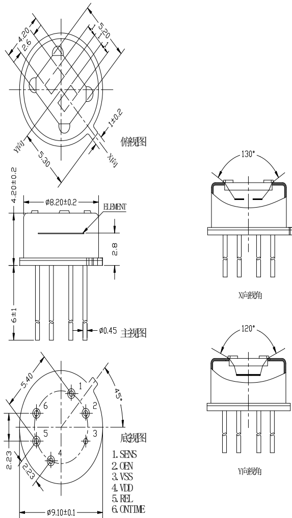
Sensor External View (UNIT: mm)
