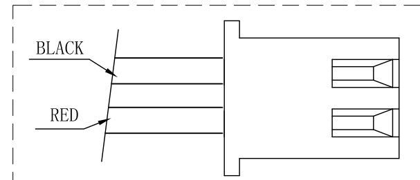
JST XHP-2 HOUSING FRONT VIEW S=2
