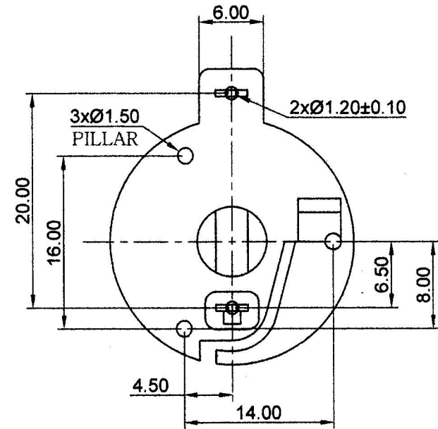
PCB MOUNTING LAYOUT
