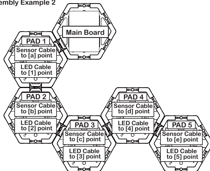
Assembly Example 2
