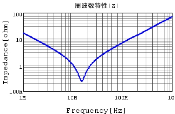
DE2E3SA103MA3BT02F |Z| DC0V, 20degC
