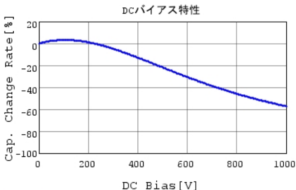
DE2E3SA103MA3BT02F C-DC bias capchange, 20.0
