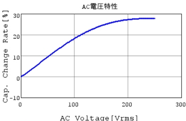
DE2E3SA103MA3BT02F C-AC Voltage capchange, I
