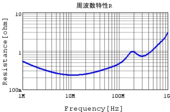
DE2E3SA103MA3BT02F R DC0V, 20degC
