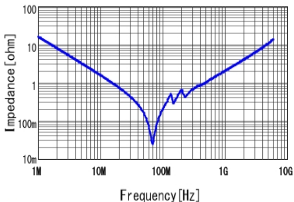
■ GRM2195C1H103JA01 |Z| DCOV, 25degC
