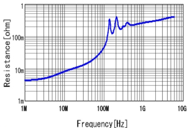
■ GRM2195C1H103JA01 R DCOV, 25degC
