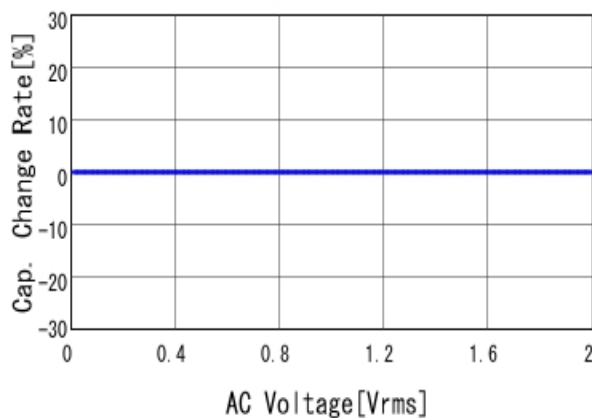
■ GRM31C5C1H224GE02 C-AC Voltage capchange, DC0V, 25.0d
