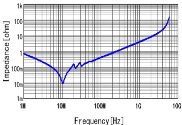
■ GRM31C5C1H224GE02 |Z| DC0V, 25degC
