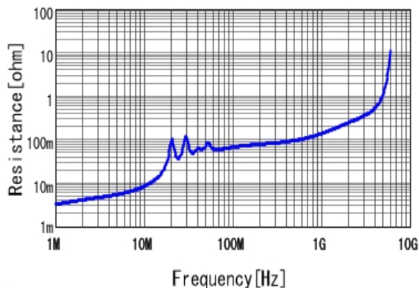
■ GRM31C5C1H224GE02 R DC0V, 25degC
