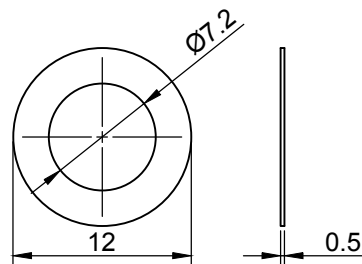
WASHER
