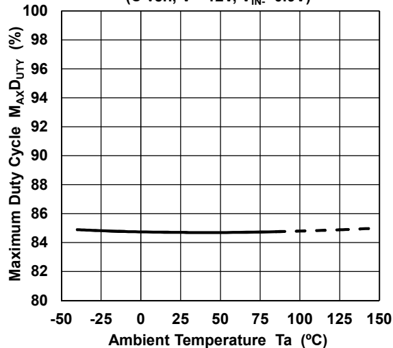
Maximum Duty Cycle vs. Temperature (C ver., V^+=12V , V_{IN}=0.9V )
