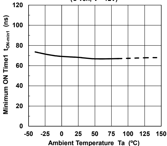
Minimum ON Time1 vs. Temperature (C ver., V^+=12V )
