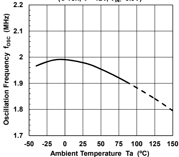
Oscillation Frequency vs. Temperature (C ver., V^+=12V , V_{IN}=0.9V )
