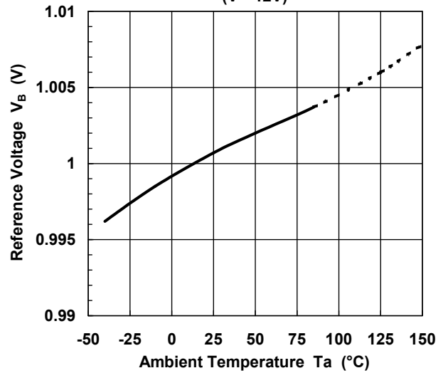
Reference Voltage vs. Temperature ( V^+=12\text{V} )
