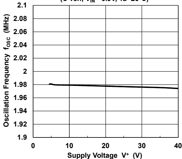
Oscillation Frequency vs. Supply Voltage (C ver., V_{IN}=0.9V , T_a=25^\circ C )
