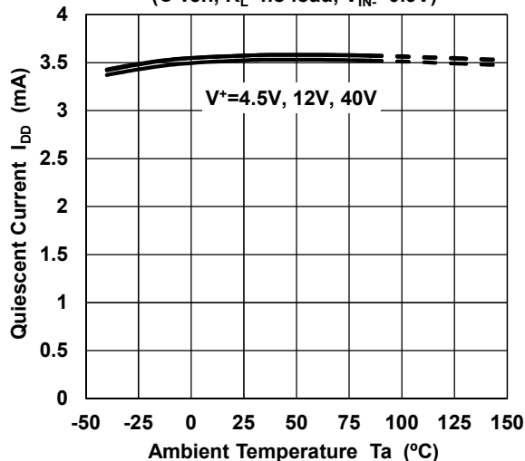
Quiescent Current vs. Temperature (C ver., R_L=no\ load , V_{IN}=0.9V )
