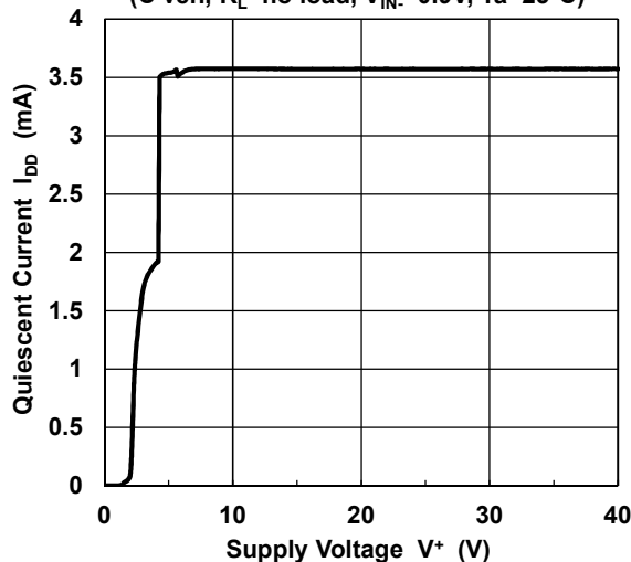
Quiescent Current vs. Supply Voltage (C ver., R_L=no\ load , V_{IN}=0.9V , T_a=25^\circ C )
