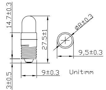
Outline Dimension
