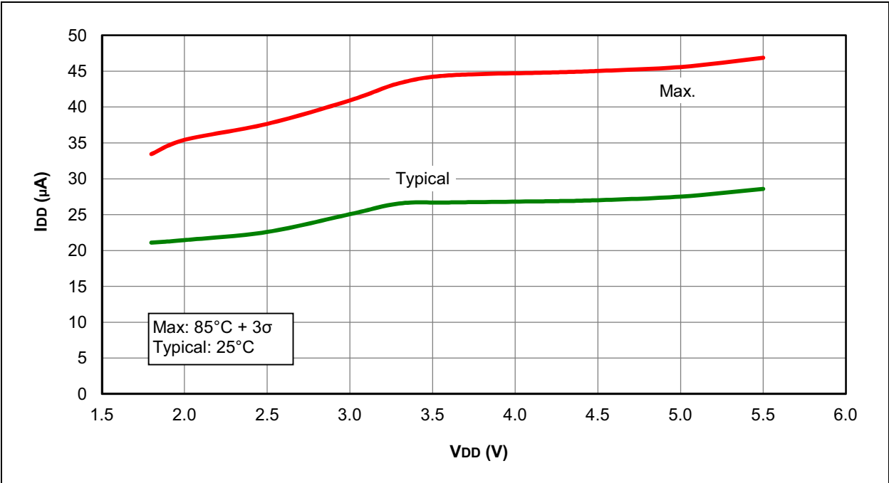
FIGURE 31-20: I_{DD} , LFINTOSC MODE ( F_{osc} = 32\text{ kHz} ), PIC12F1822 AND PIC16F1823 ONLY
