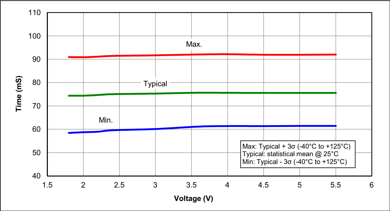
FIGURE 31-47: PWRT PERIOD
