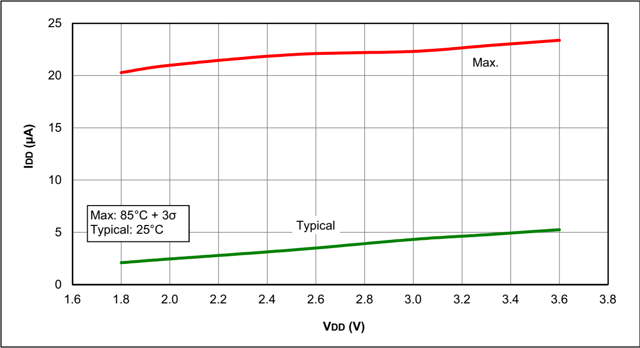
FIGURE 31-19: I_{DD} , LFINTOSC MODE ( F_{osc} = 32\text{ kHz} ), PIC12LF1822 AND PIC16LF1823 ONLY
