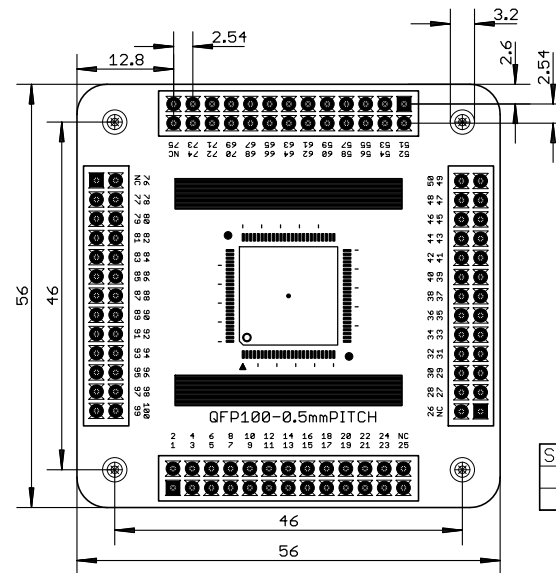
QFP100-0.5mmPITCH
