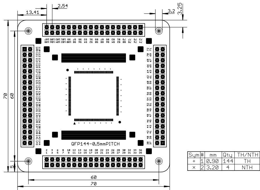
QFP144-0.5mmPITCH
