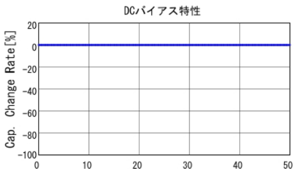
■RDE5C1H104J2K1H03B C-DC bias capchange, 25.0degC, AC1
