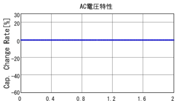
■RDE5C1H104J2K1H03B C-AC Voltage capchange, DC0V, 25.0
