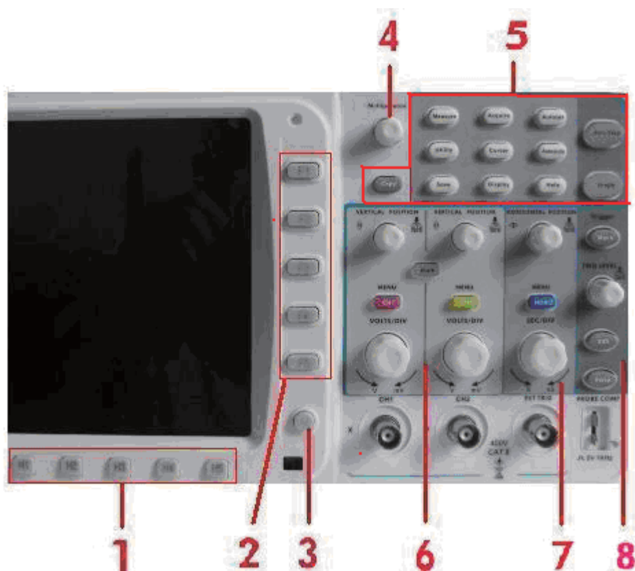
Fig. 4-5 Keys Overview
