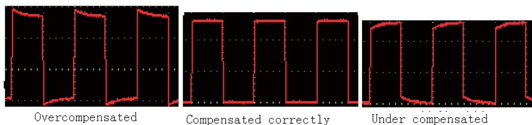
Fig. 4-8 Displayed Waveforms of the Probe Compensation
