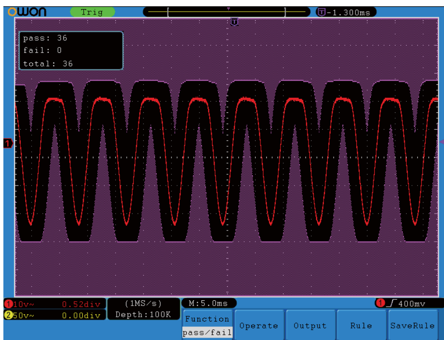
Fig.5-41 Pass/Fail test
