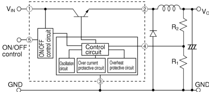
Fig.1 Step Down Voltage Output Circuit Diagram
