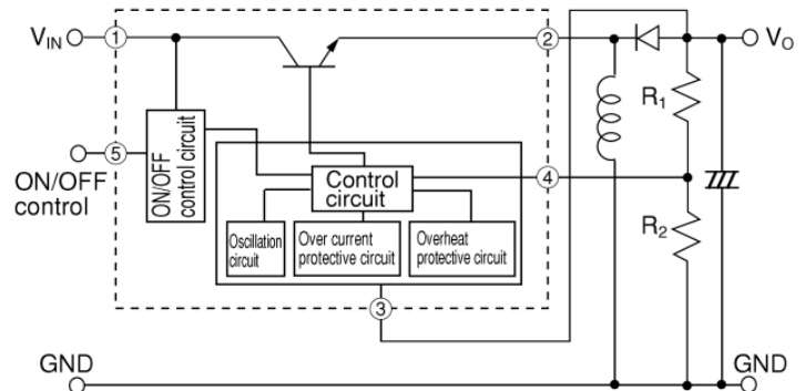
Fig.2 Inverting Output Circuit Diagram
