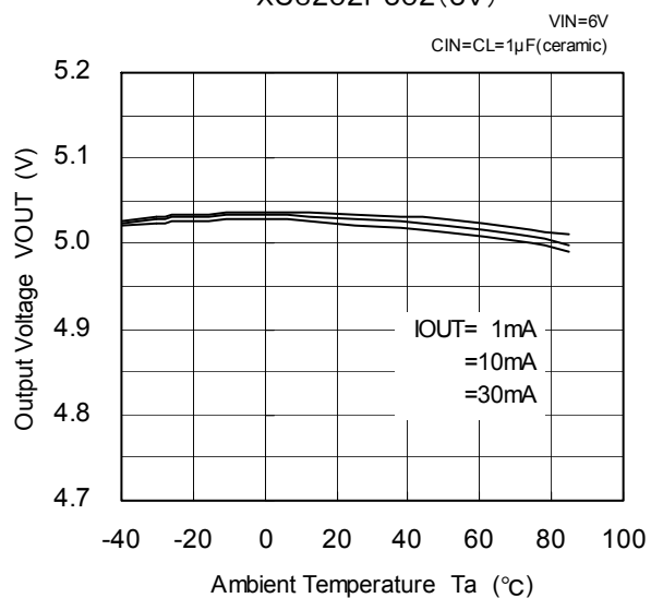
XC6202P502 (5V)
