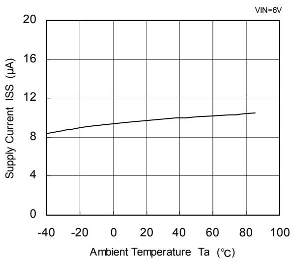
XC6202P502 (5V)
