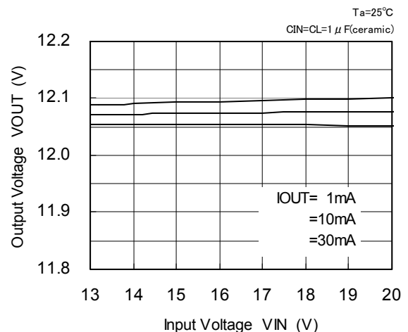
XC6202PC02 (12V 品)
