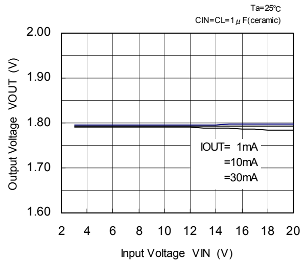
XC6202P182(1.8V)
