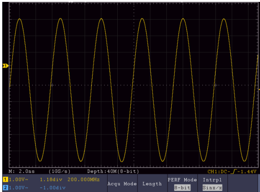
Sine(x)/x interpolation
