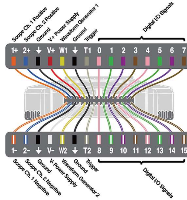
Analog Discovery 2 Pinout
