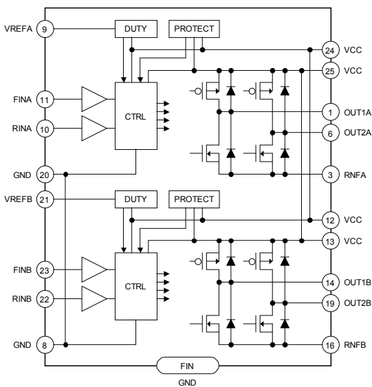
Fig.31 BD6215FP / BD6216FP
