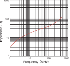
GTR-16-10-7
