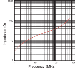
GTR-14.5-10-8
