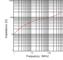
GTR-20-10-10
