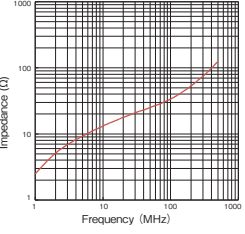
GTR-13-7-6
