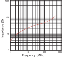
GTR-13-7-12.7
