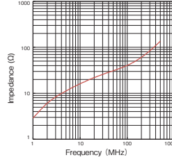
GTR-23-11-14
