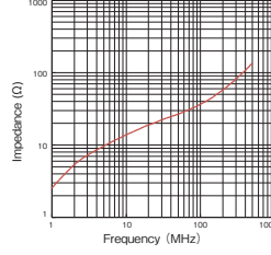
GTR-18-10-6
