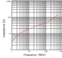
GTR-31-19-8
