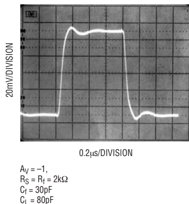
Small-Signal Transient Response
