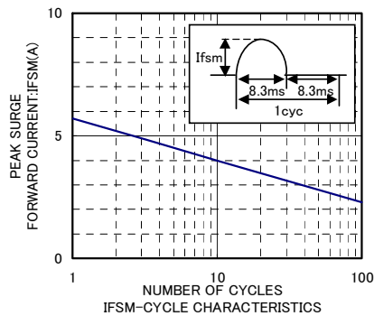
IFSM-CYCLE CHARACTERISTICS
