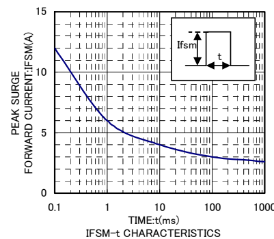
IFSM-t CHARACTERISTICS
