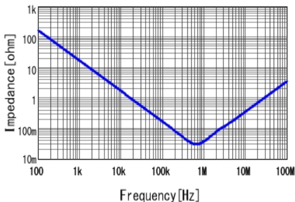
■RDEC71E106K2K1H03B |Z| DCOV, 25degC
