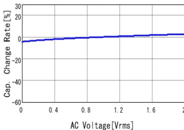
■RDEC71E106K2K1H03B C-AC Voltage capchange, DCOV, 25.0
