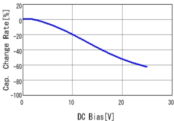
■RDEC71E106K2K1H03B C-DC bias capchange, 25.0degC, AC1
