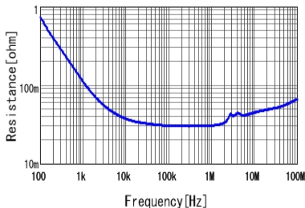
■RDEC71E106K2K1H03B R DCOV, 25degC
