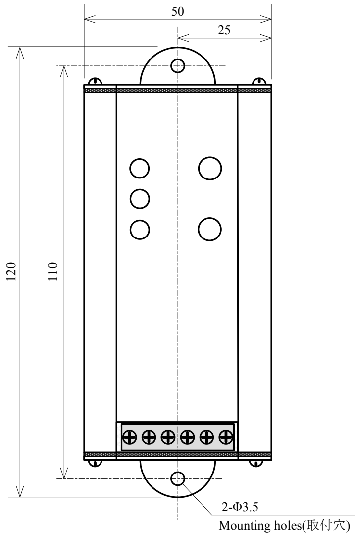
Top view (上面図)
