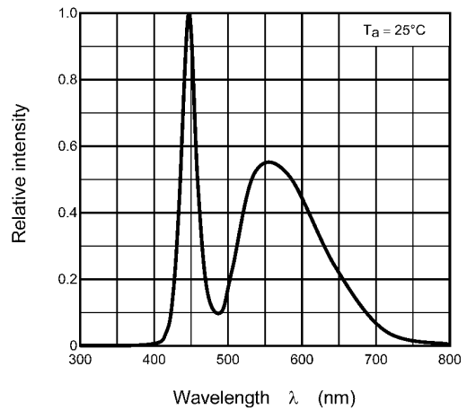
Fig. 8.4 Wavelength characteristic
