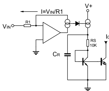
Figure 5. Rectifier Concept
