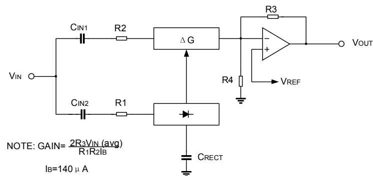
Figure 3. Basic Expander
