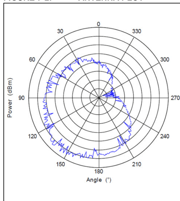
FIGURE 7-2: ANTENNA PLOT
