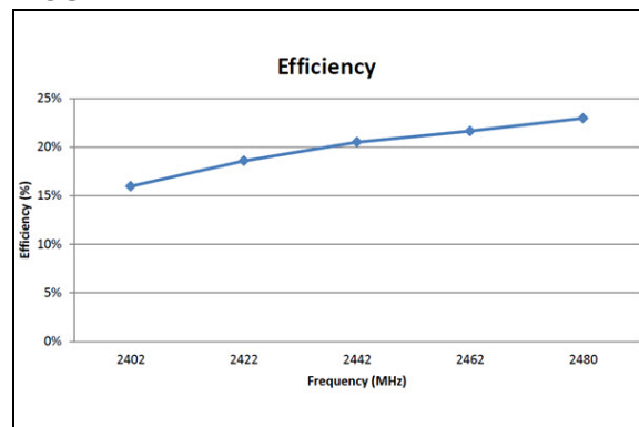
FIGURE 7-1: EFFICIENCY
