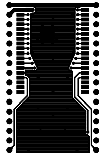
AE-ESP32-WROVER-BO TOP
