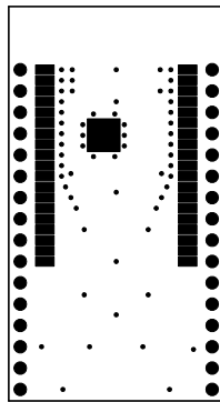
AE-ESP32-WROVER-B0 TOP-SOLDERMASK
