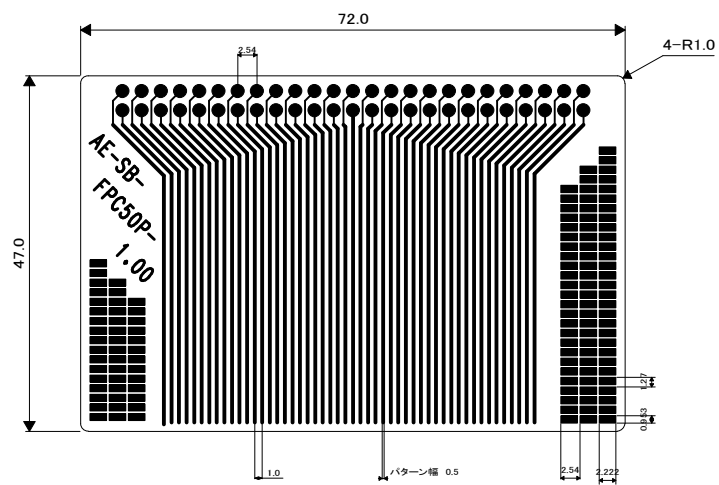
AE-SB-FPC50P-1.00 L1-PATTERN
