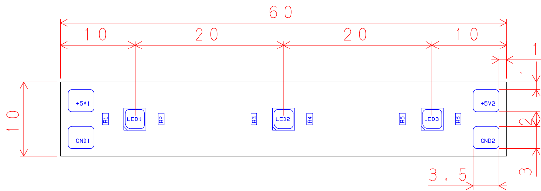
AE-SUNWHITELED1X3-5V DIMENSIONS
