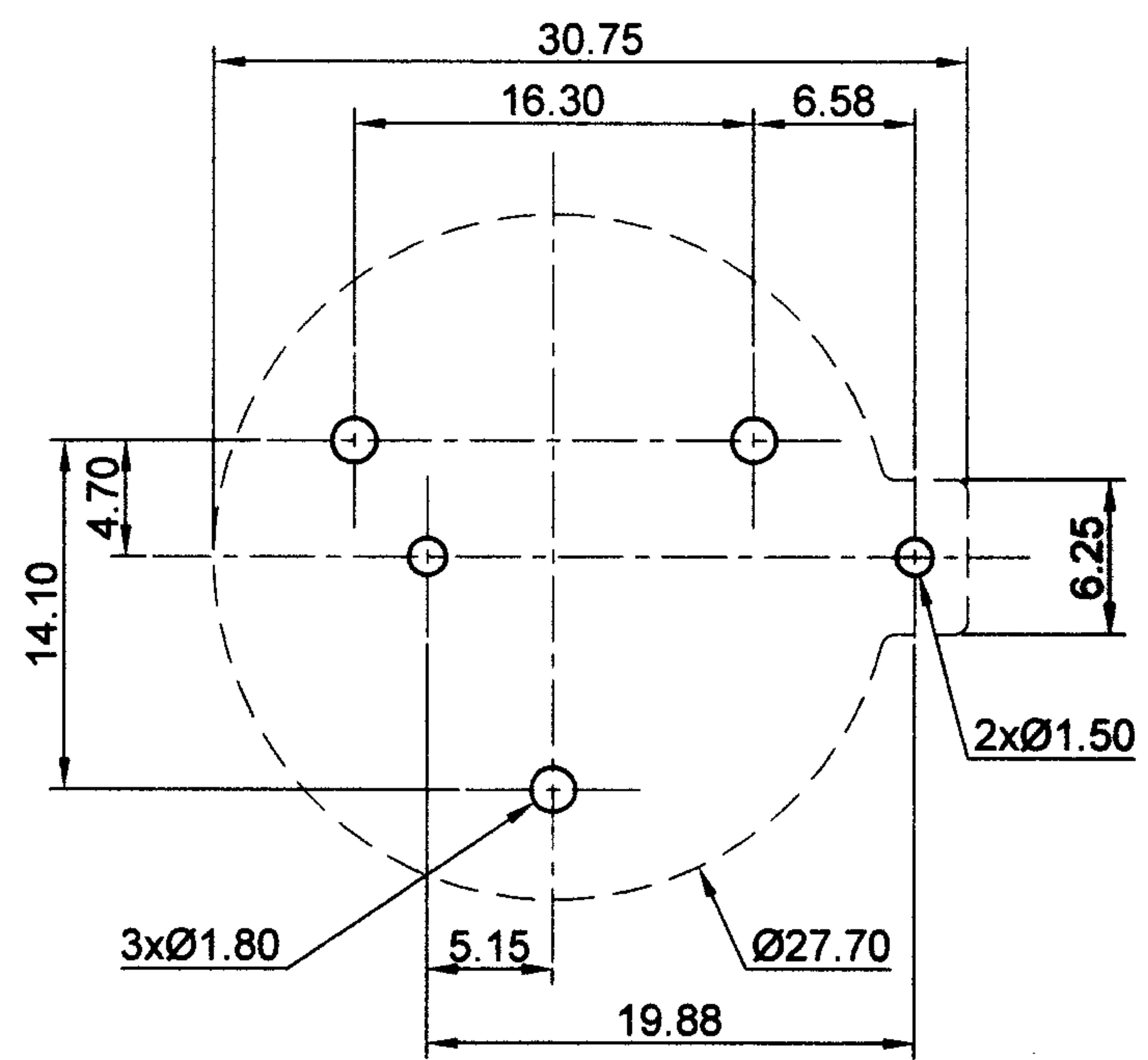
PCB MOUNTING LAYOUT
