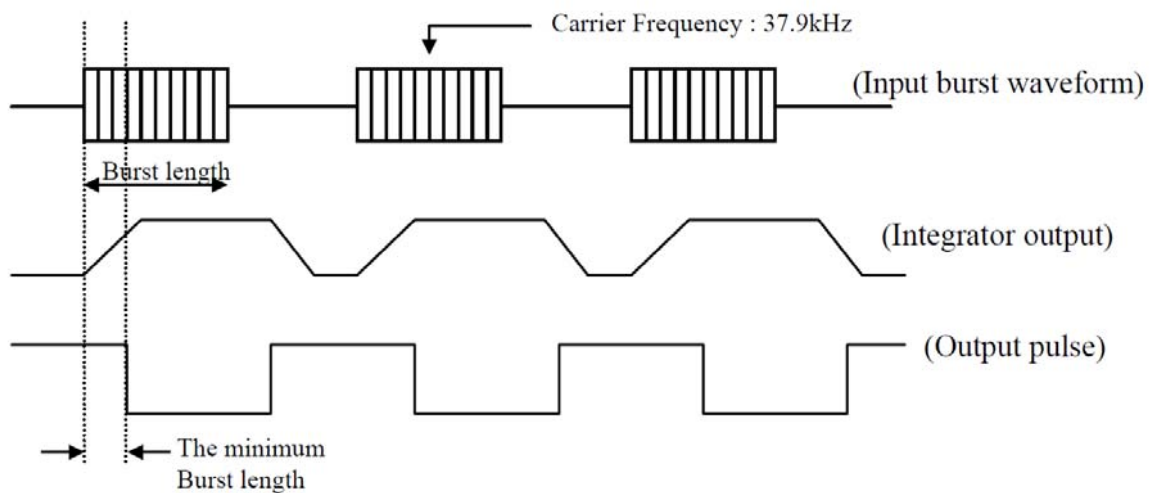
[ Fig.2 ] Transmitter
