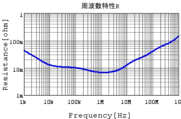
ECASD41E336M040KA0 R DCOV, 25degC
