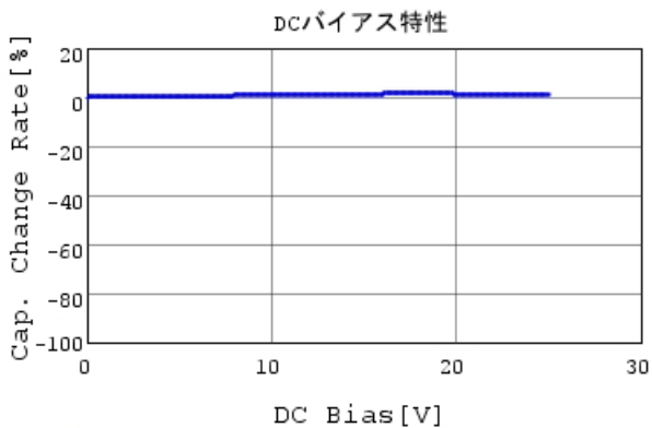
ECASD41E336M040KA0 C-DC bias capchange, 25.0
