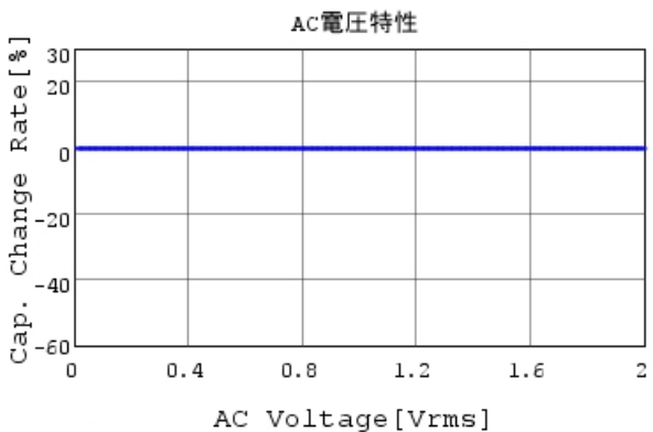
ECASD41E336M040KA0 C-AC Voltage capchange, I
