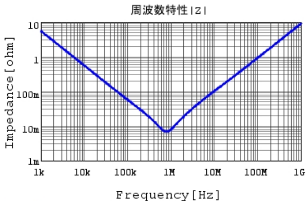
ECASD41E336M040KA0 |Z| DCOV, 25degC
