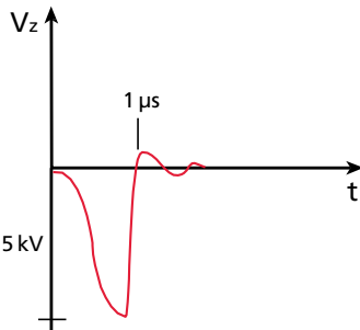
Direct series triggering
