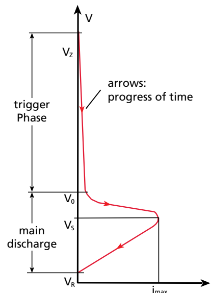
The impedance characteristic of the flash discharge
