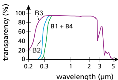
Transparency of borosilicate glasses
