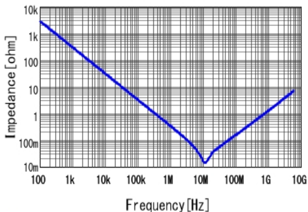
■ GRM155R61E105KA12 |Z| DCOV, 25degC
