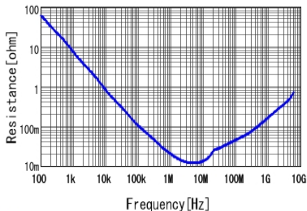
■ GRM155R61E105KA12 R DCOV, 25degC
