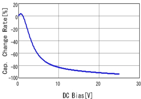
■ GRM155R61E105KA12 C-DC bias capchange, 25.0degC, AC1.
