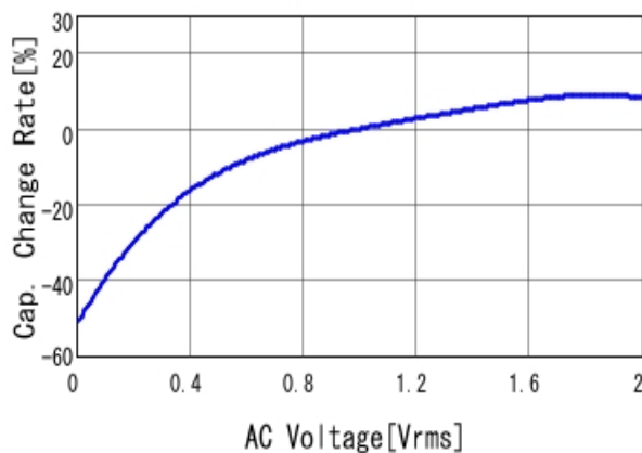
■ GRM155R61E105KA12 C-AC Voltage capchange, DCOV, 25.0d
