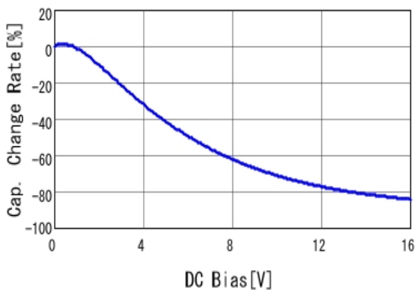
■ GRM32EC81C476KE15 C-DC bias capchange, 25.0degC, AC0.
