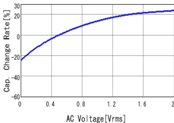
■ GRM32EC81C476KE15 C-AC Voltage capchange, DCOV, 25.0d
