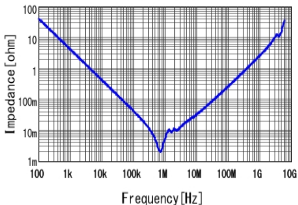
■ GRM32EC81C476KE15 |Z| DCOV, 25degC
