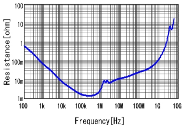
■ GRM32EC81C476KE15 R DCOV, 25degC
