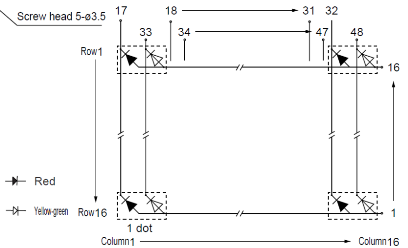
Internal connection diagram
