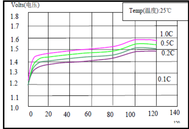
(1.0C Rate Charging Curves) 1.0C 充电曲线图
