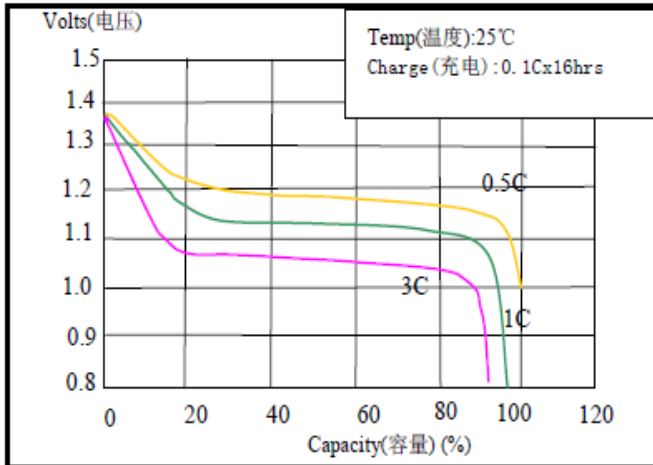
0.5C/1C/3C Rate Discharging Curves (放电曲线图)
