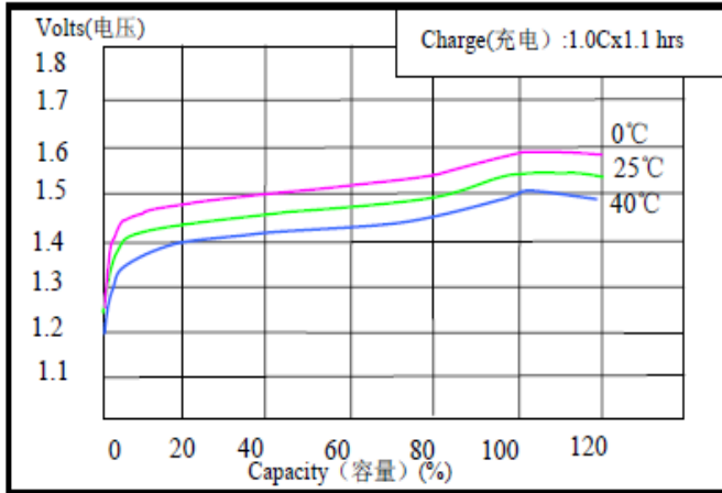
(1.0C Rate Charging Curves) 1.0C 充电曲线图
