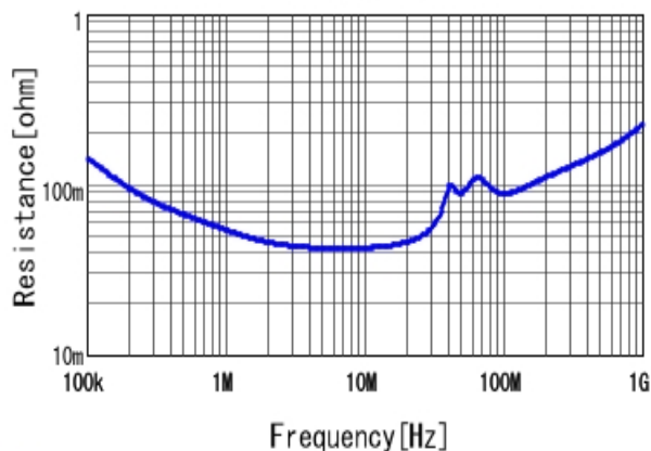
■RDER72A104K1K1H03B R DCOV, 25degC
