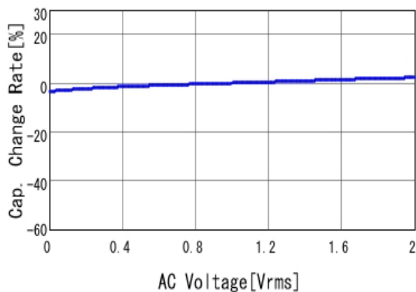
■RDER72A104K1K1H03B C-AC Voltage capchange, DCOV, 25.0
