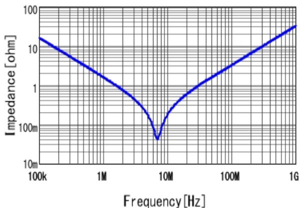
■RDER72A104K1K1H03B |Z| DCOV, 25degC
