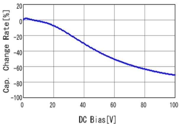
■RDER72A104K1K1H03B C-DC bias capchange, 25.0degC, AC1
